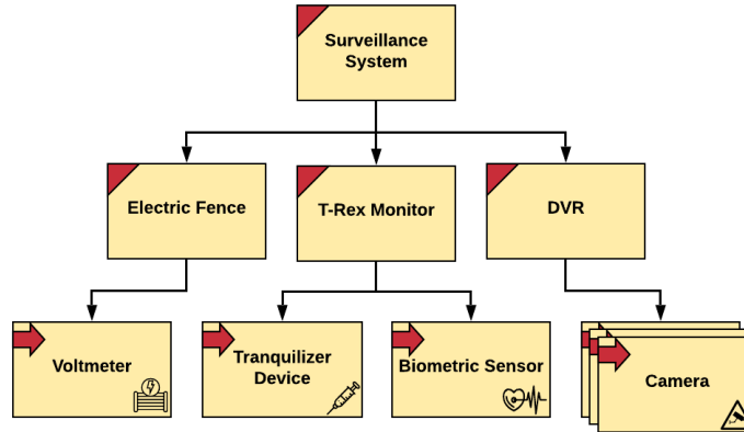
Figure 4: The Surveillance System encapsulates the Camera network (shown as a stack), the Electric Fence , and the T-Rex Monitor .
