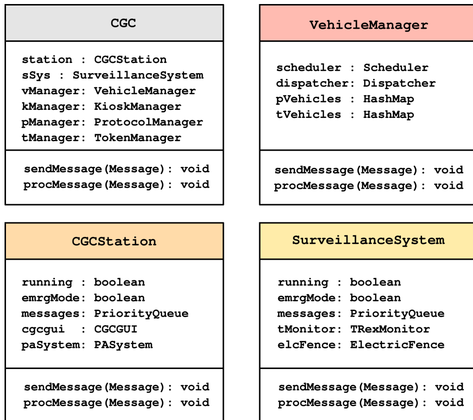
Figure 8: Uppermost Classes: The CGC acts as a server for forwarding messages between components and is the parent of the others. The VehicleManager deals with the coordination and tracking of all vehicles, the CGCStation is the component with which employees directly interact as it provides the visualization of the others, and the SurveillanceSystem manages cameras and the TRexMonitor.
